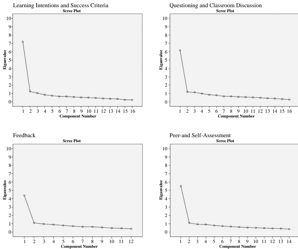
Figure 1. Scree plots from factor analysis of for the four AfLAI scales.
